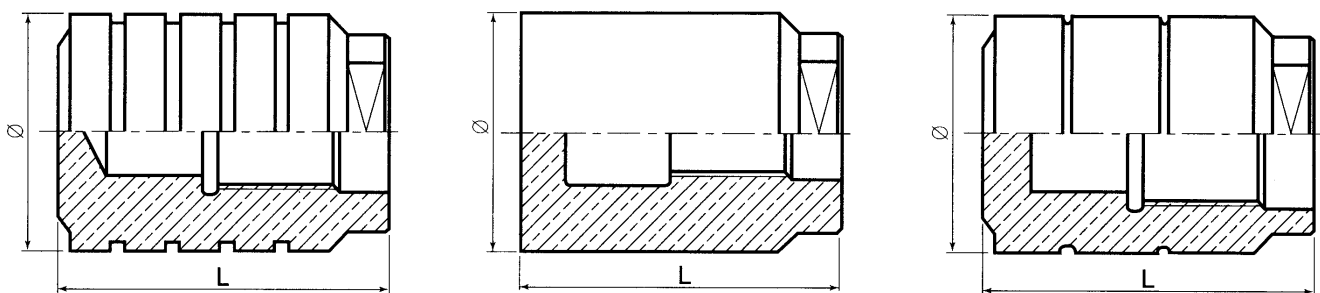
Samples of injection plunger design
